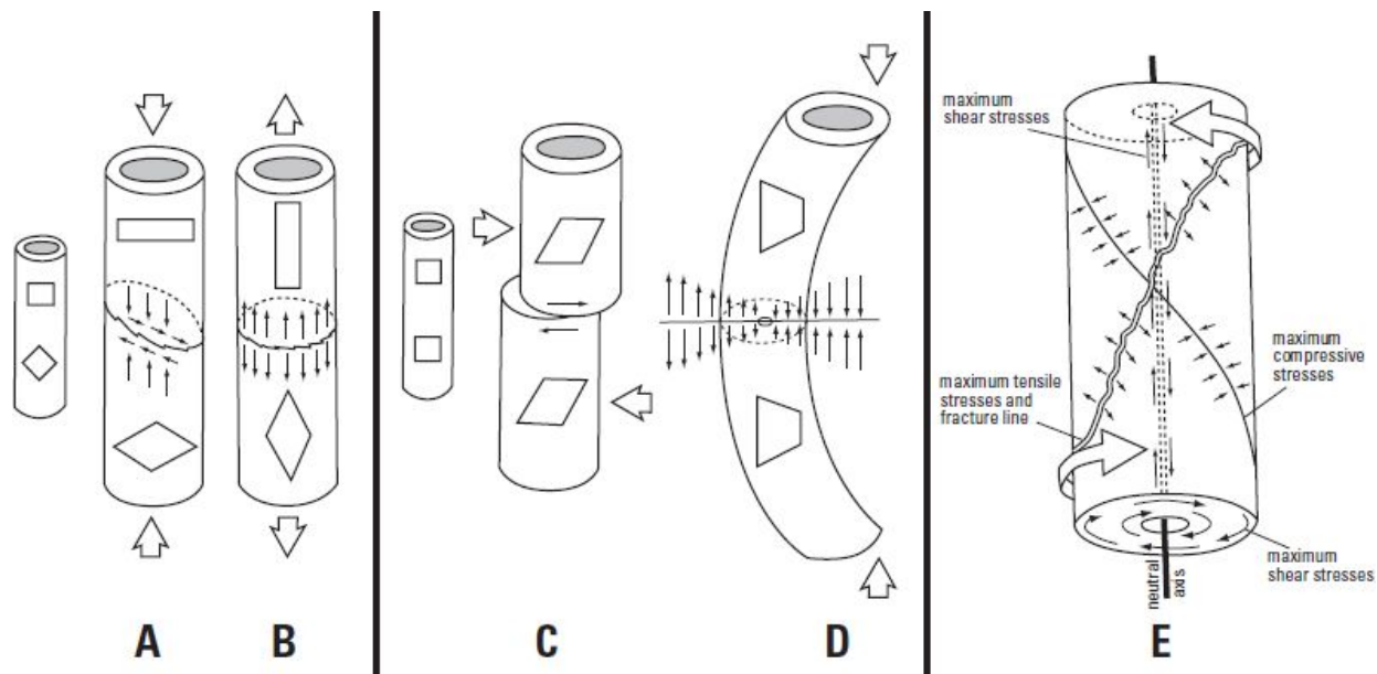
Figure 108-12. Illustration depicting stresses and strains produced by various loading modes on a cylindrical long bone. A, Compressive loading induces compressive and shear stresses and strains that, if excessive, may induce a short oblique fracture. B, Tensile loading induces tensile stresses and strains, which if excessive, induce a transverse fracture. C, Shear loading induces internal shear stresses and strains causing angular deformations. D, Bending loading induces tensile stresses and strains along the convex surface and compressive stresses and strains along the concave surface. There is a continuous gradient from maximal tensile stress, to neutral, to maximal compression. E, Torsional loading induces shear, tensile, and compressive stresses and strains, which if excessive, produce a typical spiral fracture configuration.
