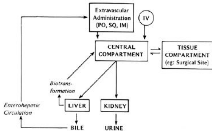
Figure 12-1. Schematic diagram of a drug's disposition in the body. PO, Per os; SQ, subcutaneous; IM, intramuscular; IV, intravenous.
