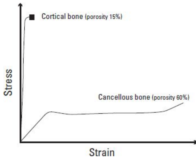
Figure 108-9. Idealized compressive stress-strain curve of cortical and cancellous bone samples depicting the effect of bone porosity on bone's mechanical behavior. Note that porous cancellous bone exhibits elastic behavior prior to its yield point. Following yield, progressive collapse of the bony trabeculae produces a long plateau of plastic deformation followed by a region of increased stiffness as the fractured trabeculae are compressed. This behavior allows cancellous bone to absorb great amounts of energy and tolerate significant strain prior to failure. Conversely, cortical bone, with its low porosity, displays brittle behavior where it is capable of tolerating great amounts of stress in the elastic region of the curve, but then fails abruptly.
