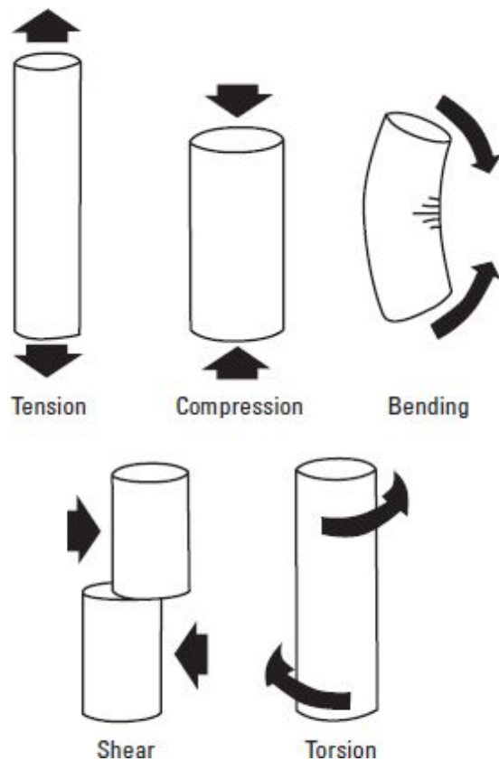
Figure 108-11. Schematic illustration of tensile, compressive, bending, shear, and torsional loading modes.
