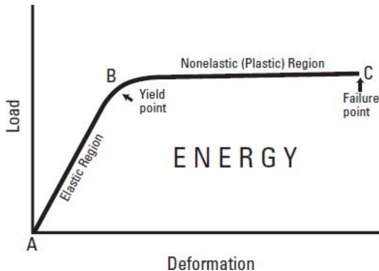
Figure 108-3. A theoretical load-deformation curve for a whole bone. Under conditions of low-level loading (elastic region, A-B), the structure deforms in direct relation to the applied load and returns to its original shape when the load is removed. Loading past the yield point (B) induces permanent deformation of shape (plastic region, B-C) even when the load is removed. If loading is progressively increased, the bone will grossly fail (fracture) at the ultimate failure point (C). The slope of the elastic region of the load-deformation curve indicates the stiffness of the studied bone. The area under the curve indicates the amount of energy absorbed by the bone prior to failure.
