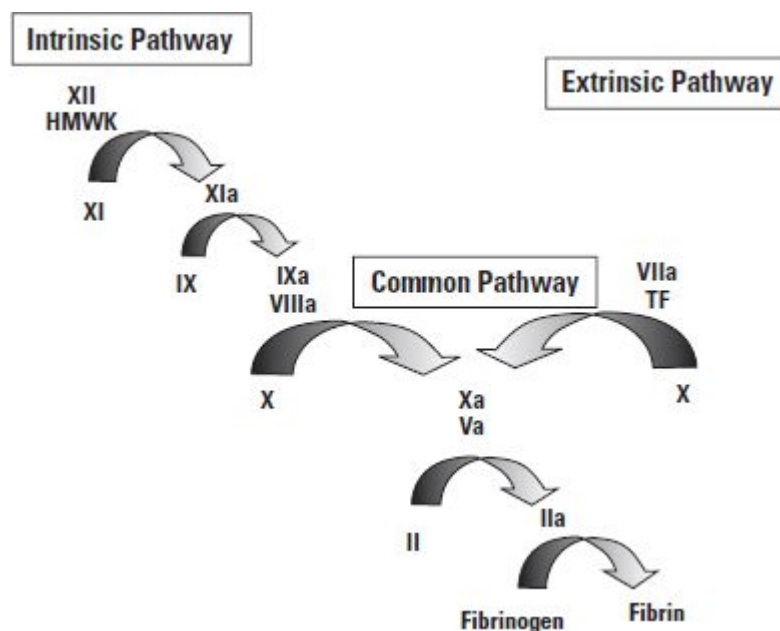
Figure 4-1. Classic coagulation cascade depicting reactions involved in the intrinsic, extrinsic, and common pathways, culminating in the production of the fibrin clot. HMWK = High molecular weight kalikrein, TF = tissue factor.
