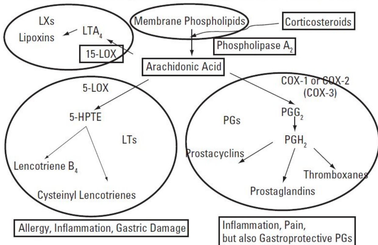
Figure 116-7. Products and enzymes of arachidonic acid metabolism.
