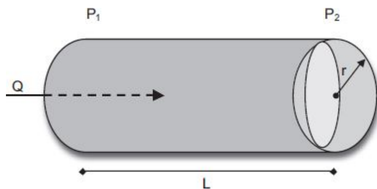
Figure 52-2. Schematic representation of Poiseuille's ( Q = \pi r^4 P / 8 \eta L ) law where Q = flow rate, r = radius of the tube, L = Length of the tube, P = pressure within the tube, and \eta = viscosity.
